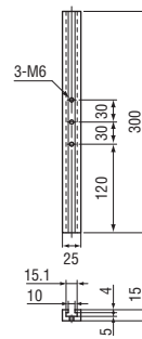
C Universal chuck slide base
